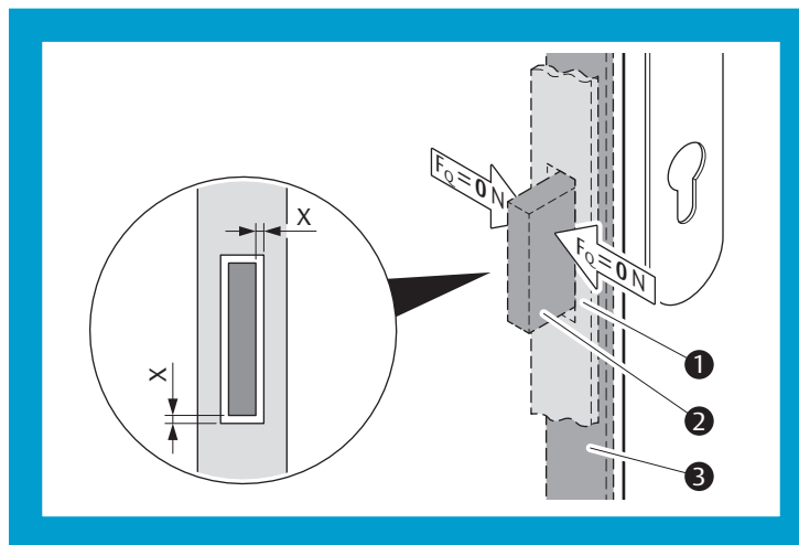
Fig. 7: Bolt is free of transverse loads ( F_Q )
