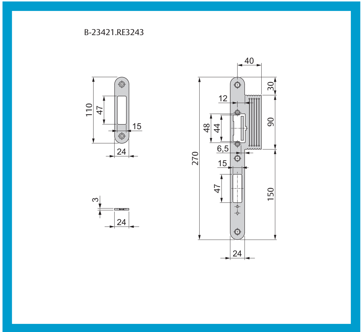
Fig. 8: Strike plates for wood
